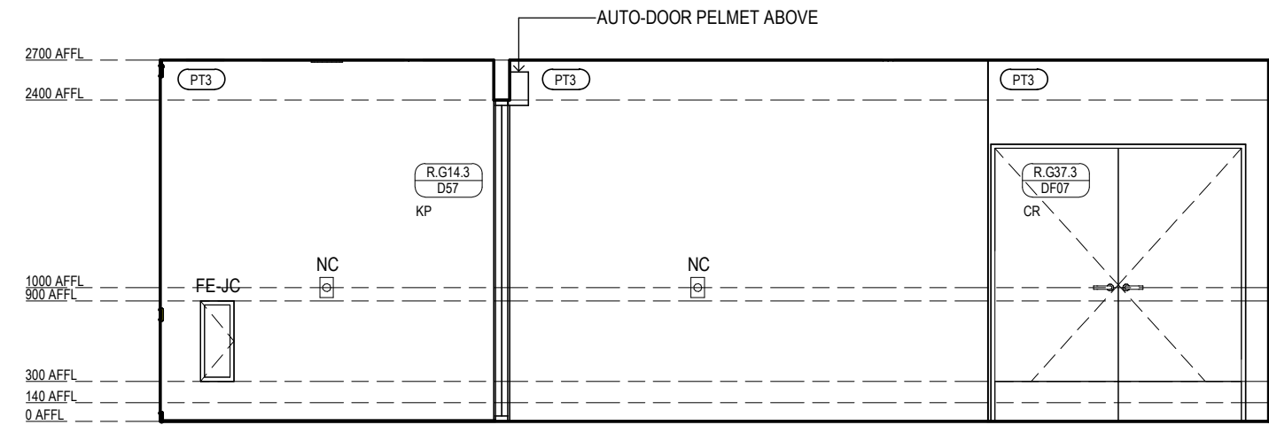
VILLAGE HEALTH & WELLNESS - AIRLOCK & WAITING ELEVATION 2 Scale 1: 50
