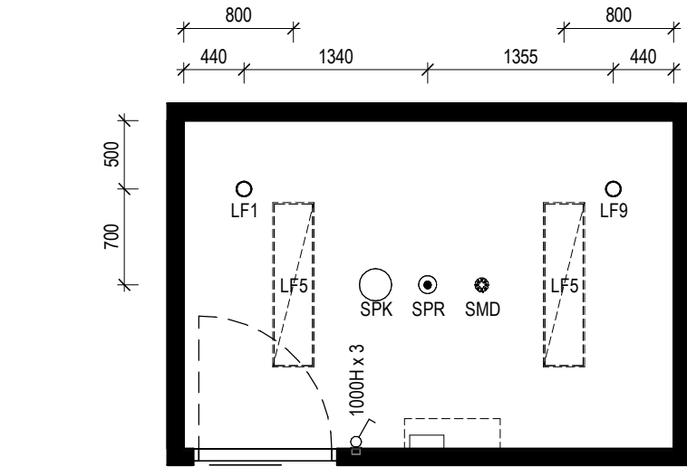
4 RCP - VILLAGE HEALTH & WELLNESS - CONSULT 2 Scale 1: 50
